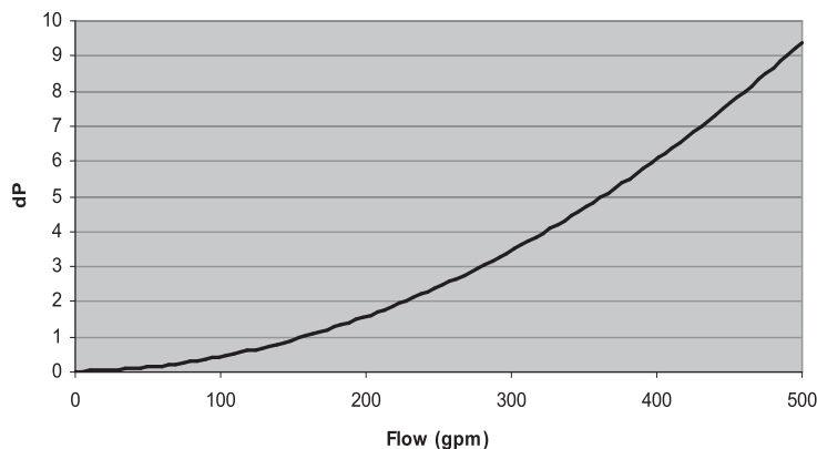
Flow vs dP (2.9" Cartridge Inlet Orifice)
